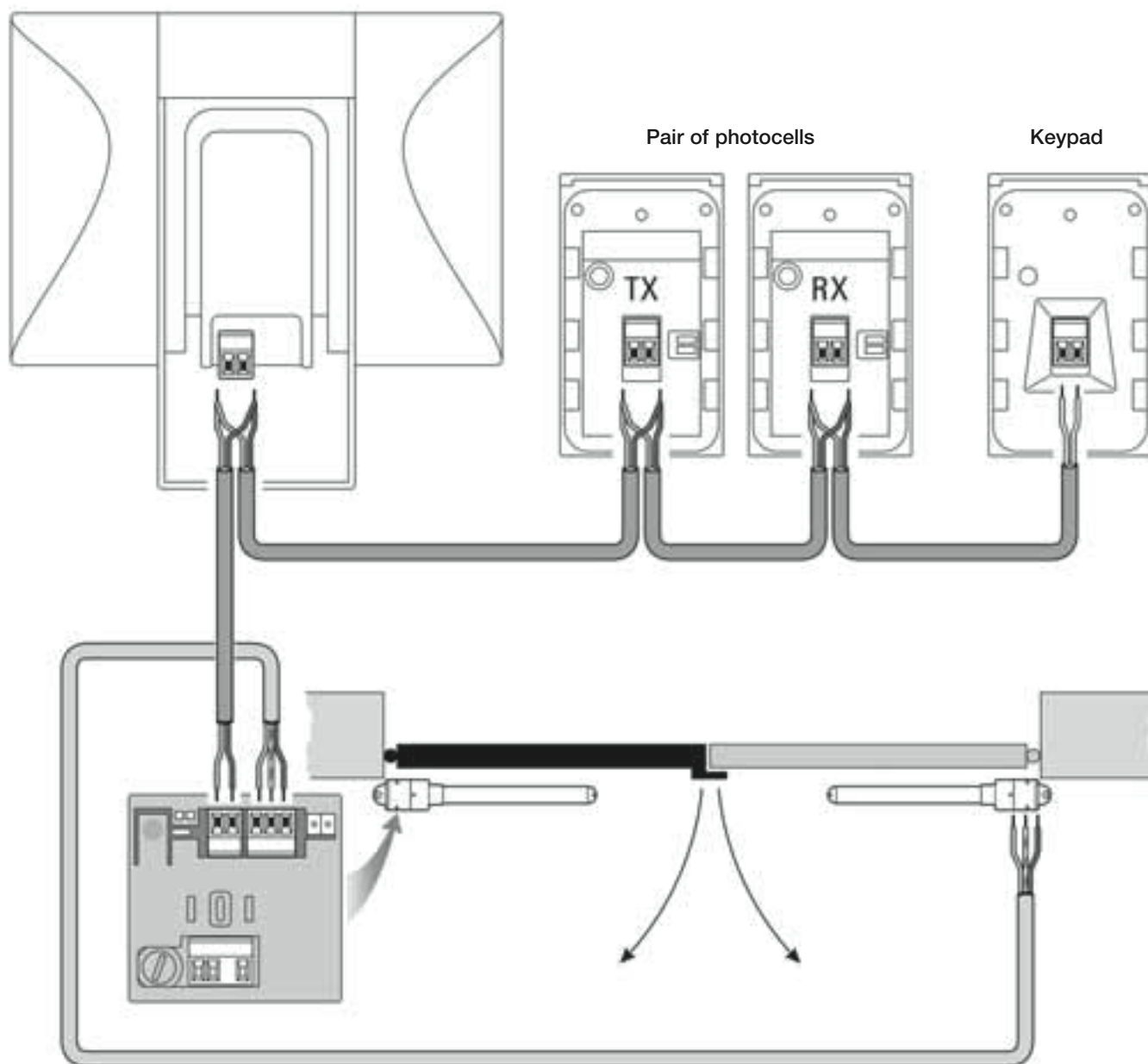
Flashing light
